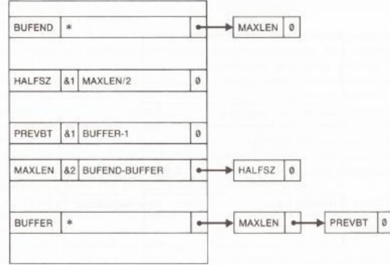
3 PREVBT EQU BUFFER-1
