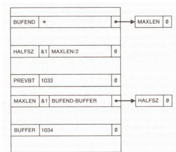
4 BUFFER RESB 4096
