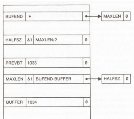
4 BUFFER RESB 4096
